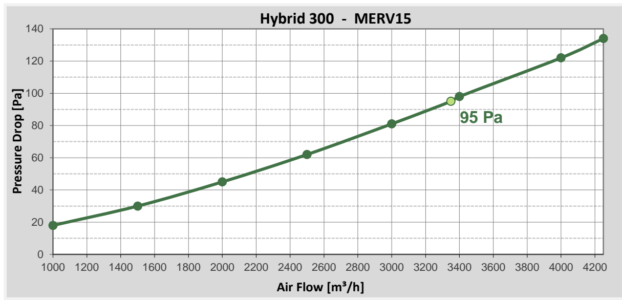
Panelfilter 592x592x296 mm @ 3350 m³/h
