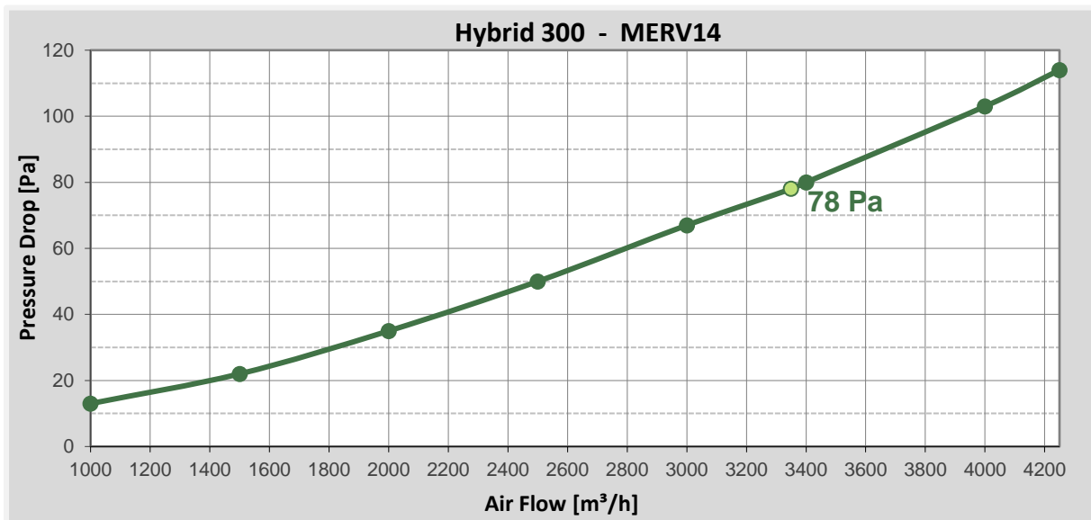
Panelfilter 592x592x296 mm @ 3350 m³/h
